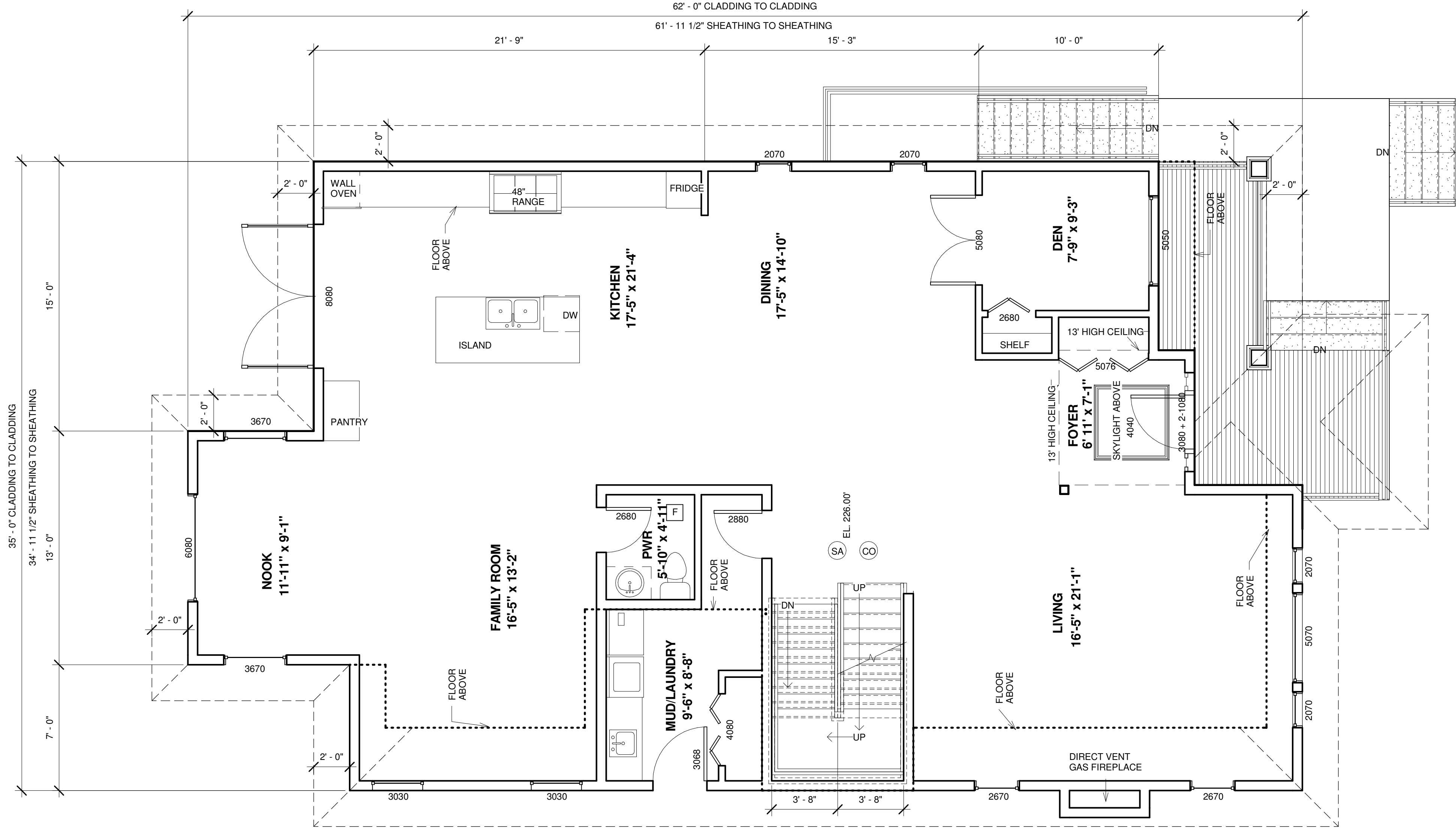
MAIN FLOOR PLAN-1873.0 SQ.FT./COVER AREAS 148.28 SQ.FT.
